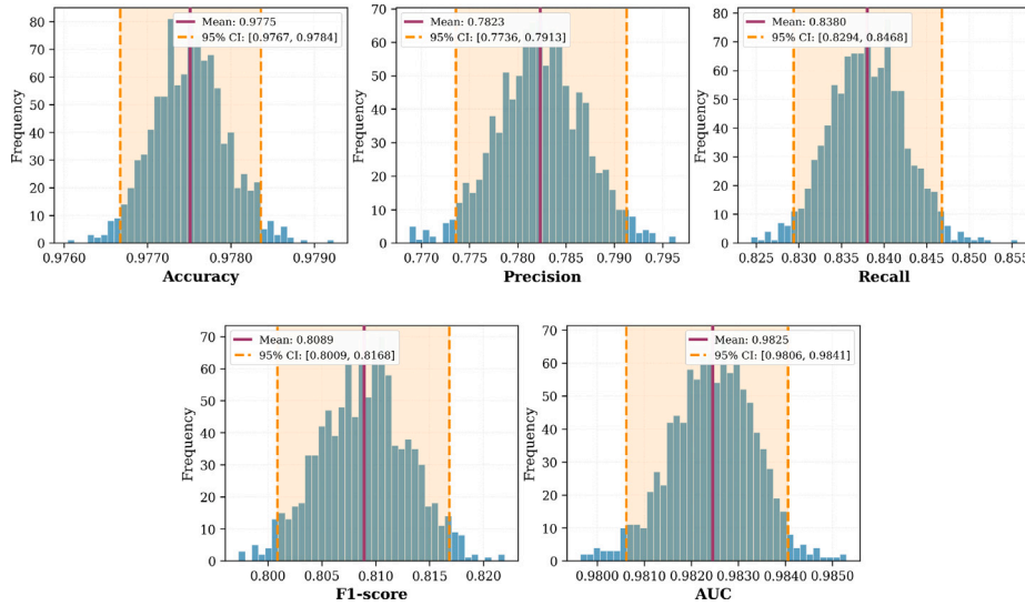
Fig. 4. Metrics distribution after bootstrap validation on random forest for binary classification.
